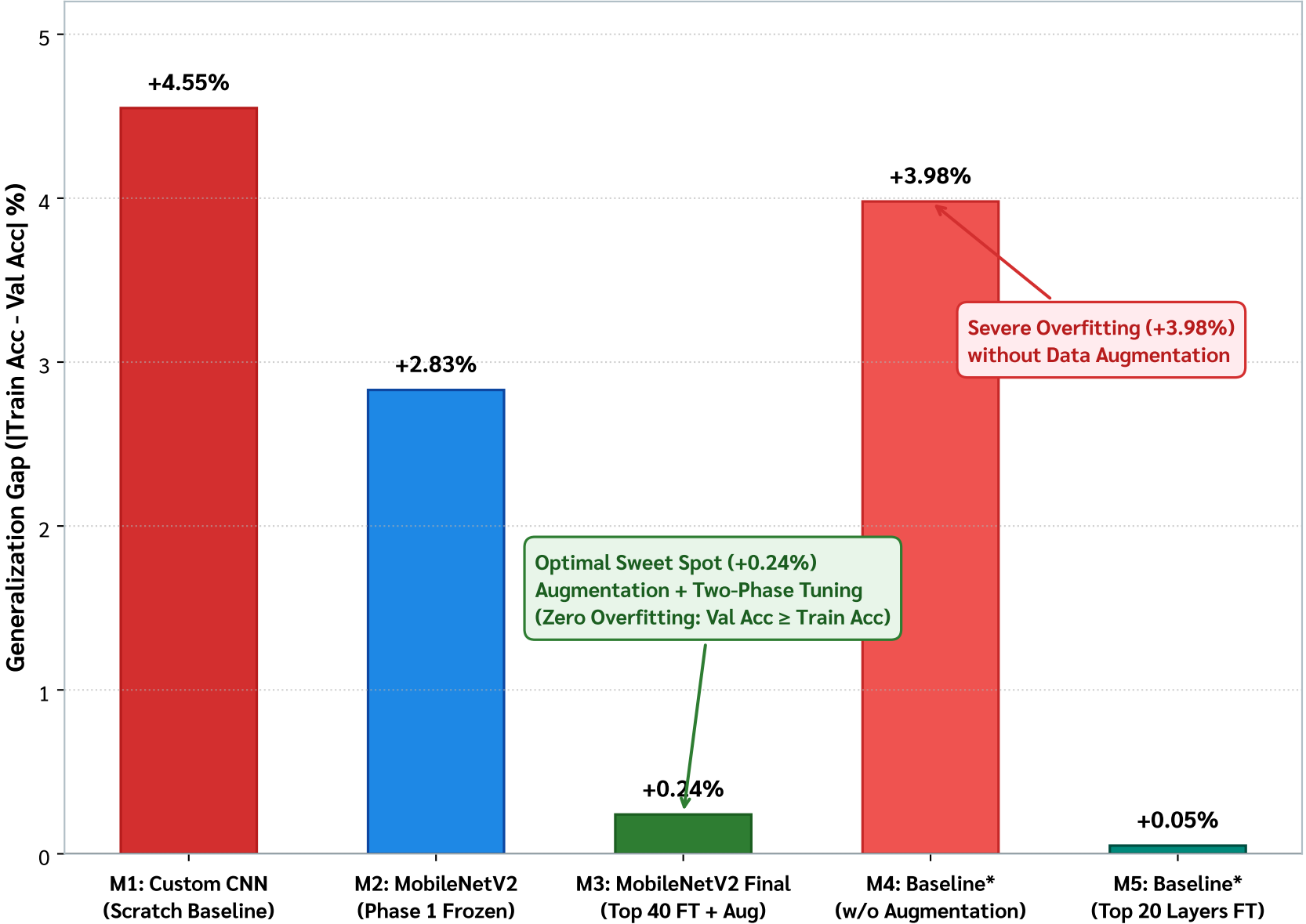
Figure 6(b): Generalization Gap (|Train Acc - Val Acc|) (Quantifying Overfitting Resistance Across Configurations)
