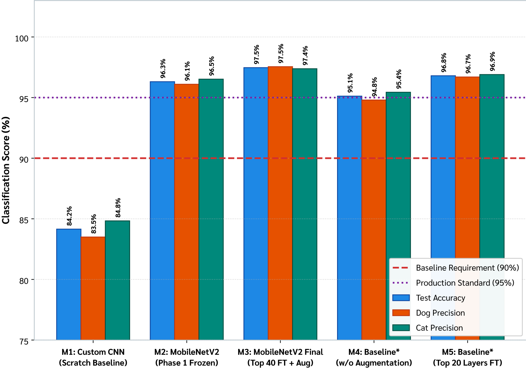
Figure 6(a): Ablation Benchmark Across 5 Model Configurations (Final-Test Accuracy & Class Precision Scores)
